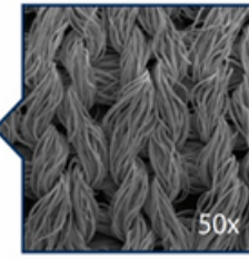
Polyester Wipes
